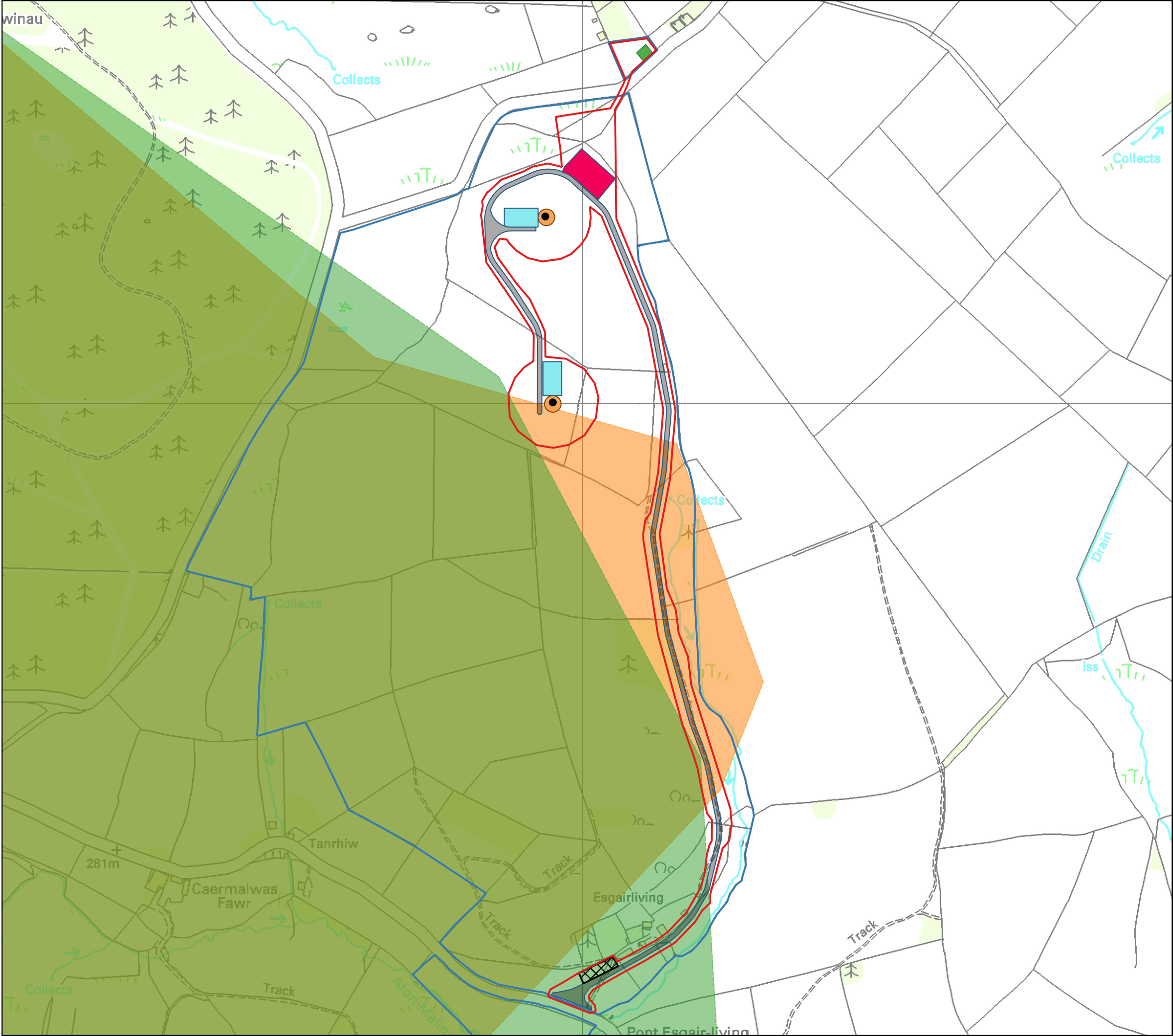
Figure 2.1: Strategic and Pre-Assessed Areas for Wind
