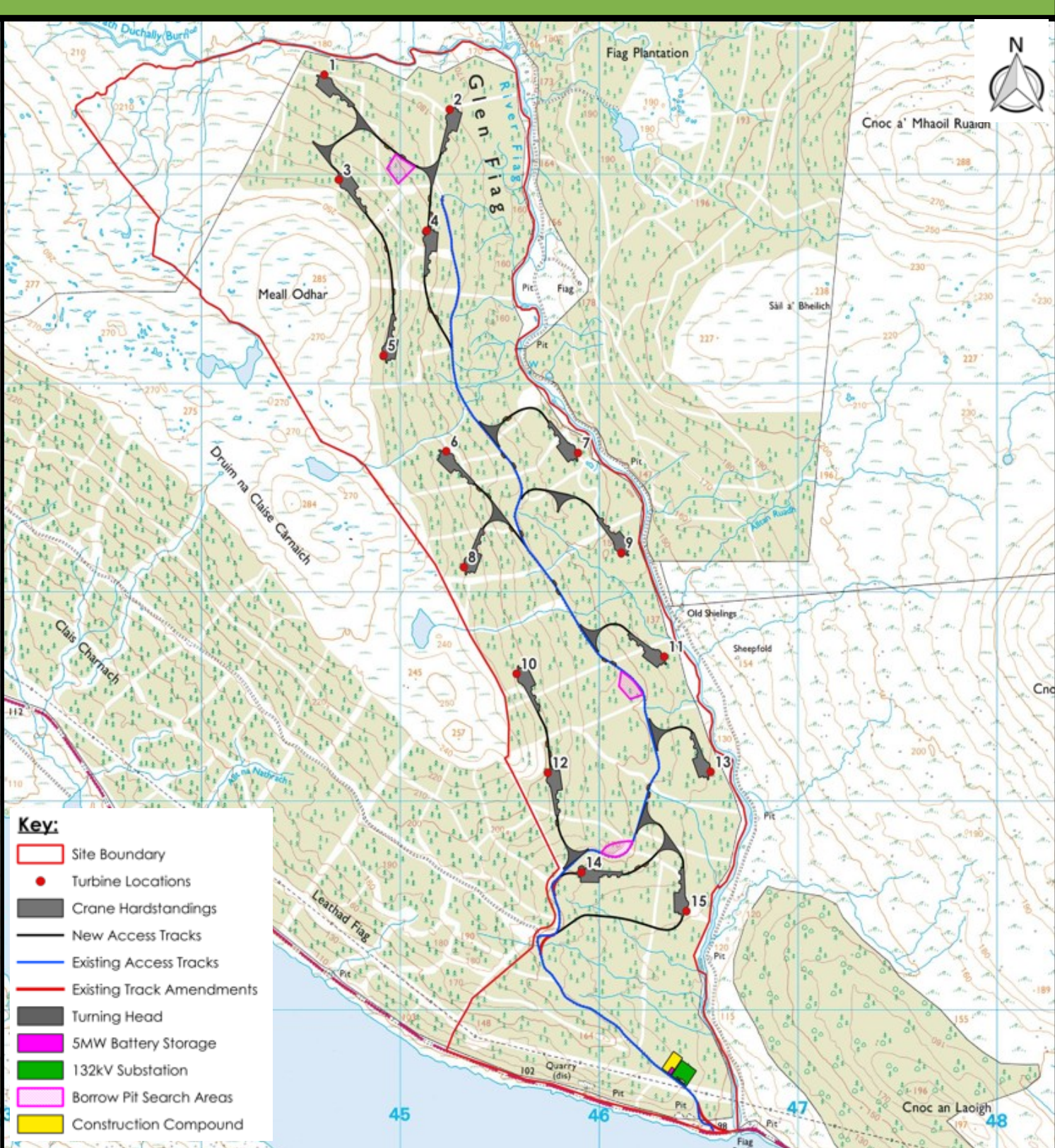
Revised Layout 2
