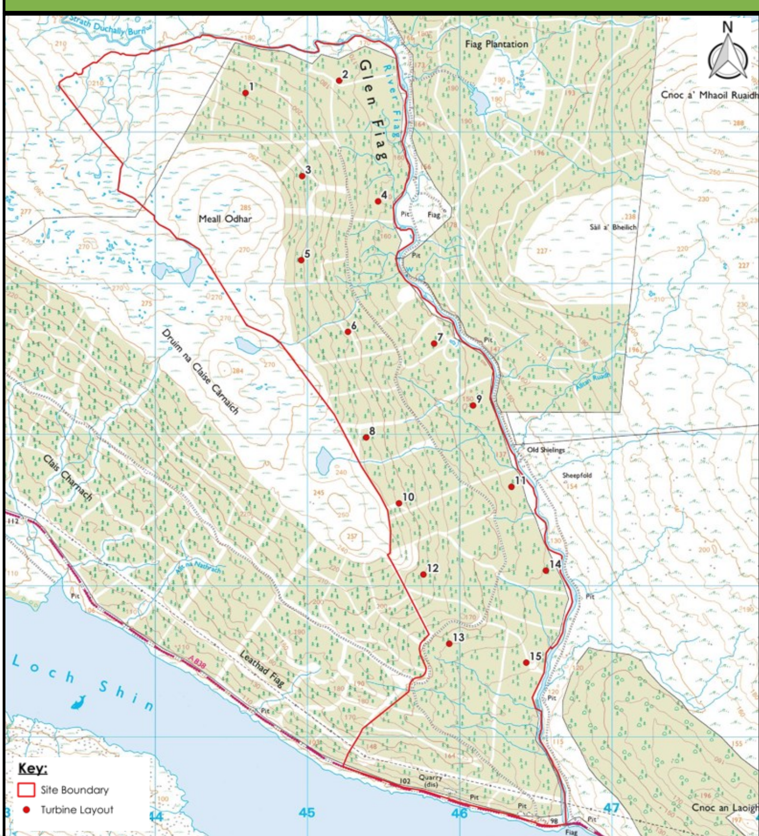
Revised Layout 1
