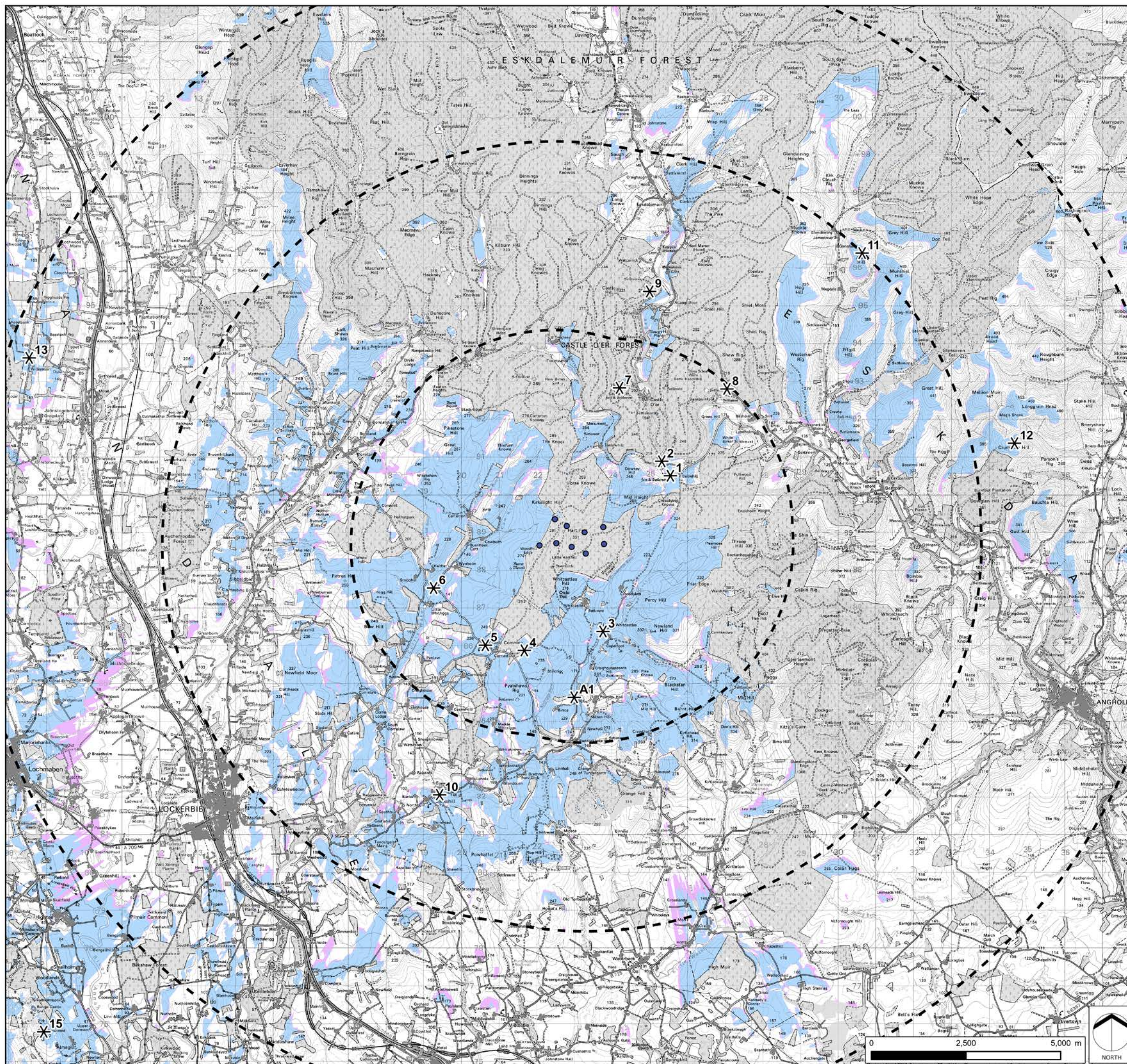
FIGURE 3 Comparative ZTV to Blade Tip with Screening Effect of Woodland and Settlement: Consented and Proposed Layouts
