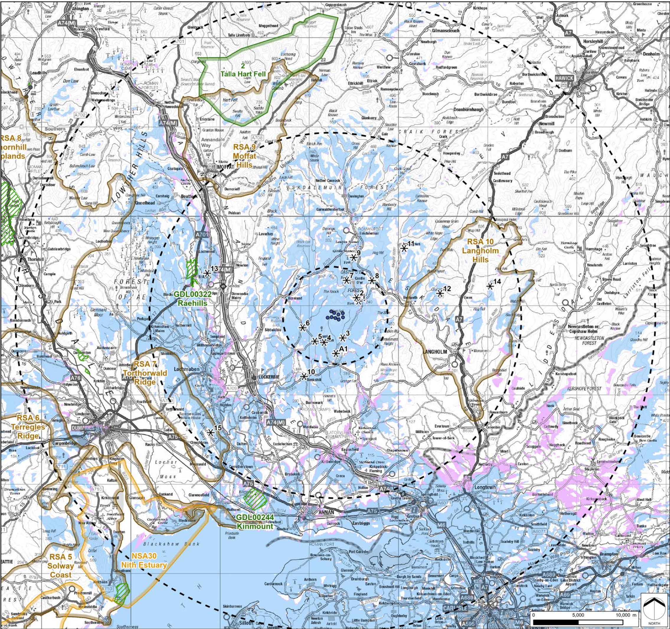
FIGURE 2 Comparative ZTV to Blade Tip: Consented and Proposed Layouts
