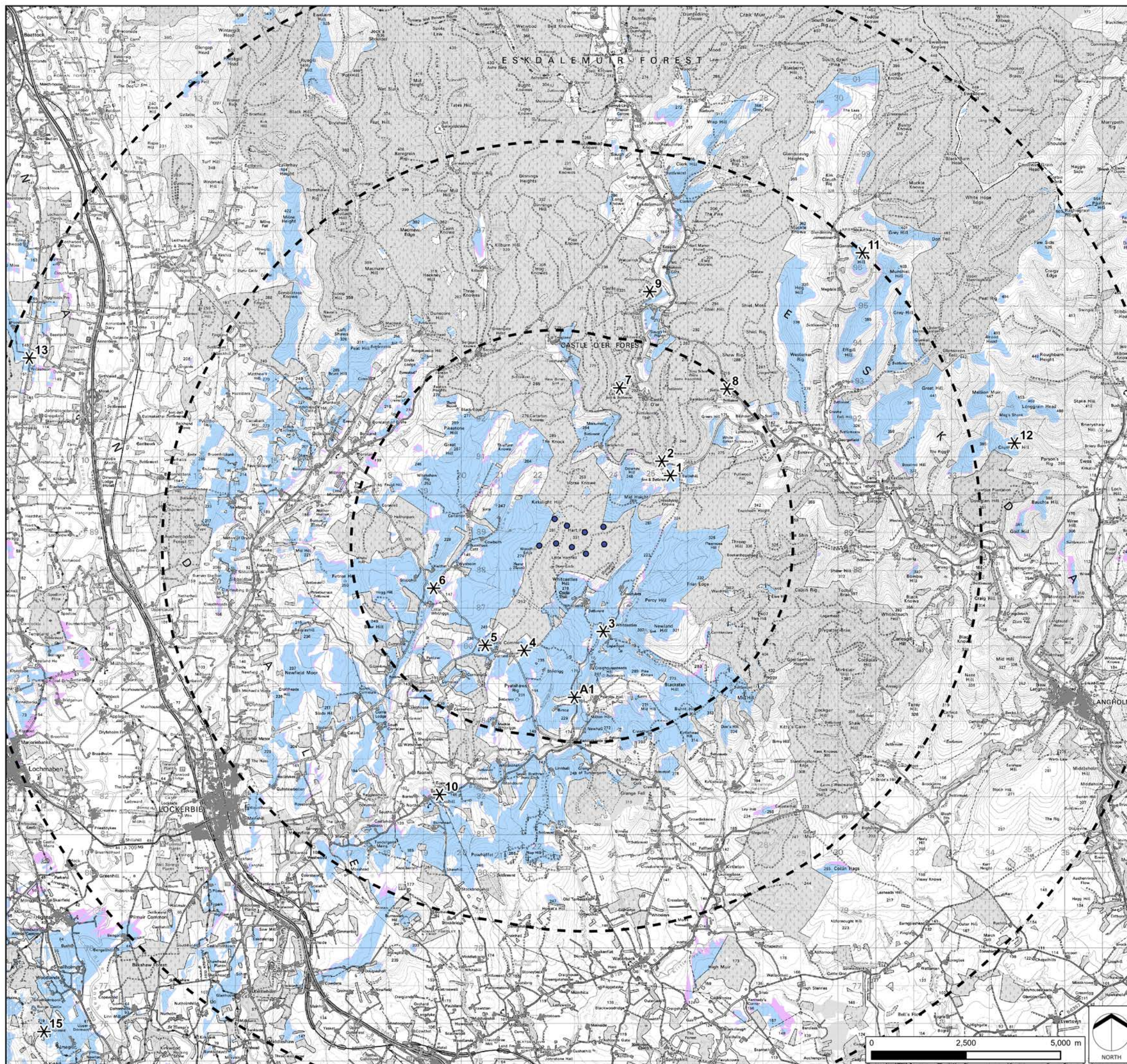
FIGURE 8 Comparison ZTV: Lighting on Consented and Proposed Layouts
