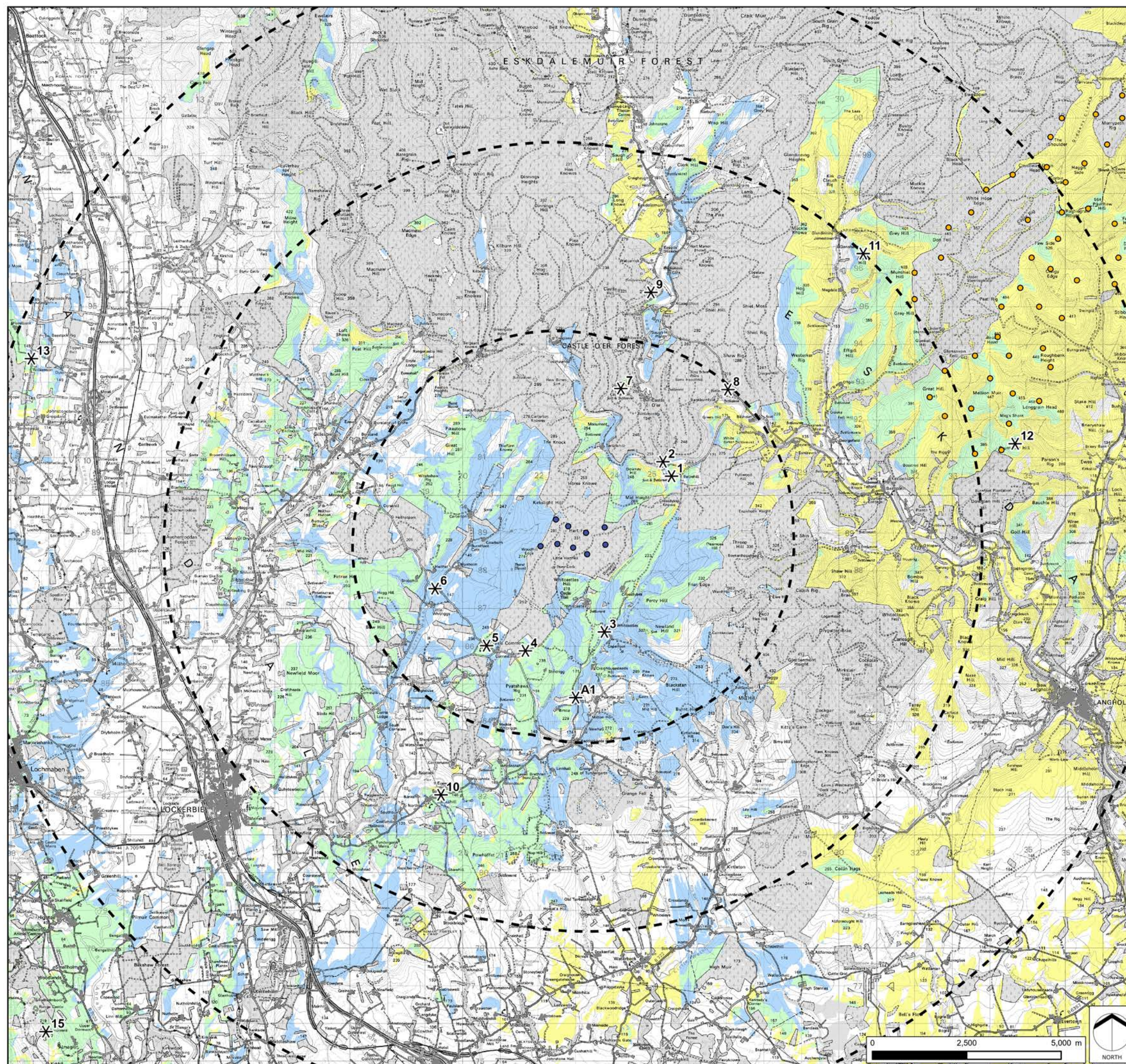
FIGURE 5 Cumulative ZTV to Blade Tip with Screening Effect of Woodland and Settlement: Faw Side and Little Hartfell
