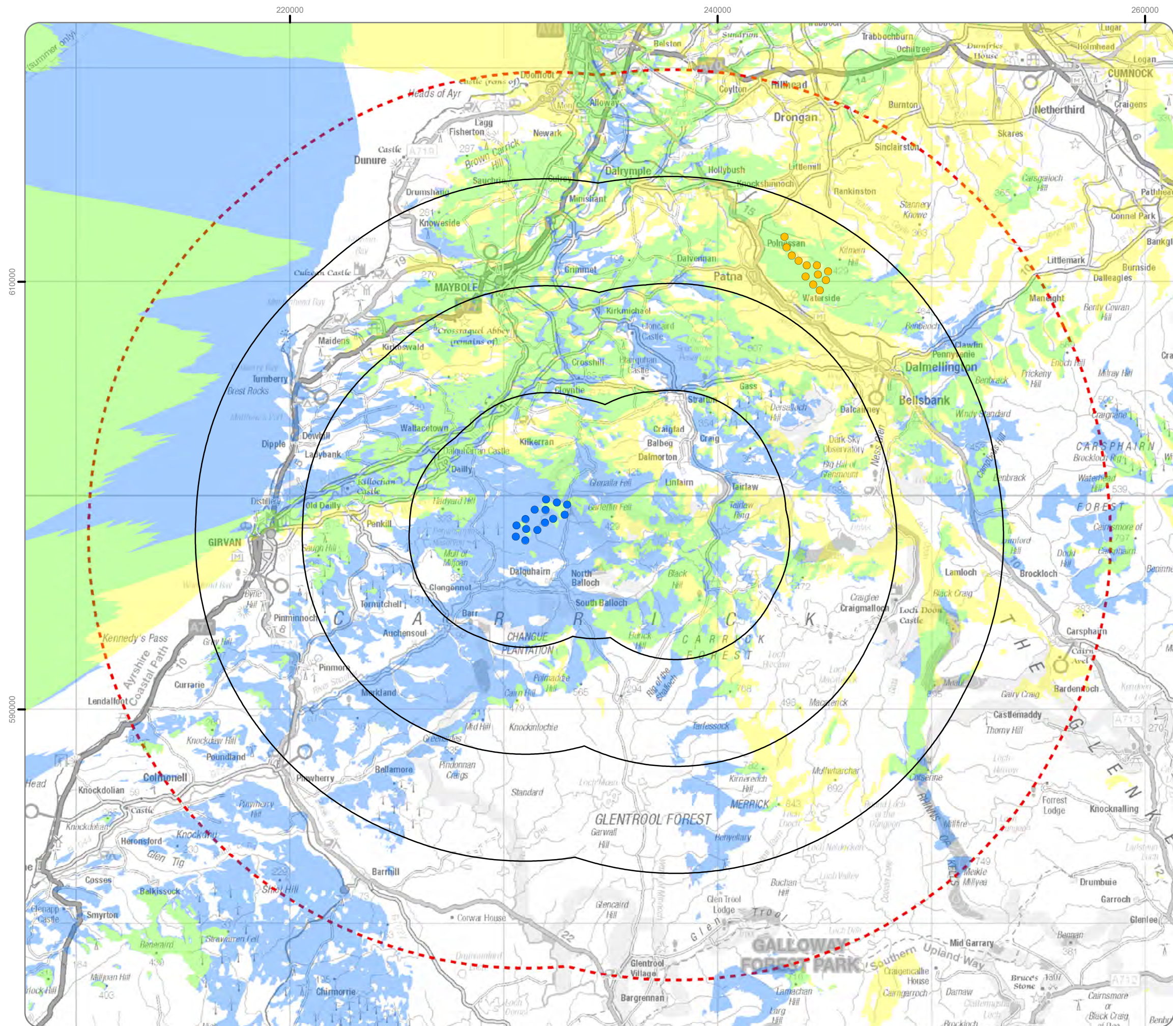
Figure AI 8 Cumulative ZTV Craiginmoddie with Knockkippen
