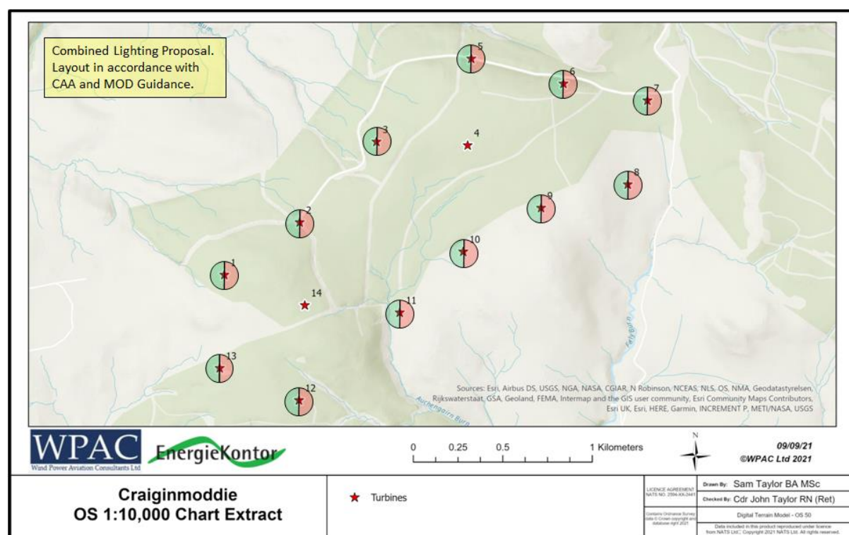
Figure 6 Combined CAA and MOD Lighting Diagram
