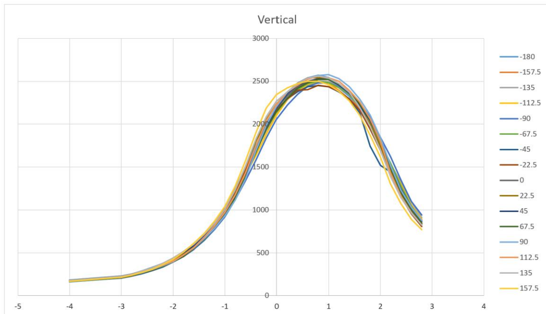
Figure 12 (MI GAM Light Measurement Results)
