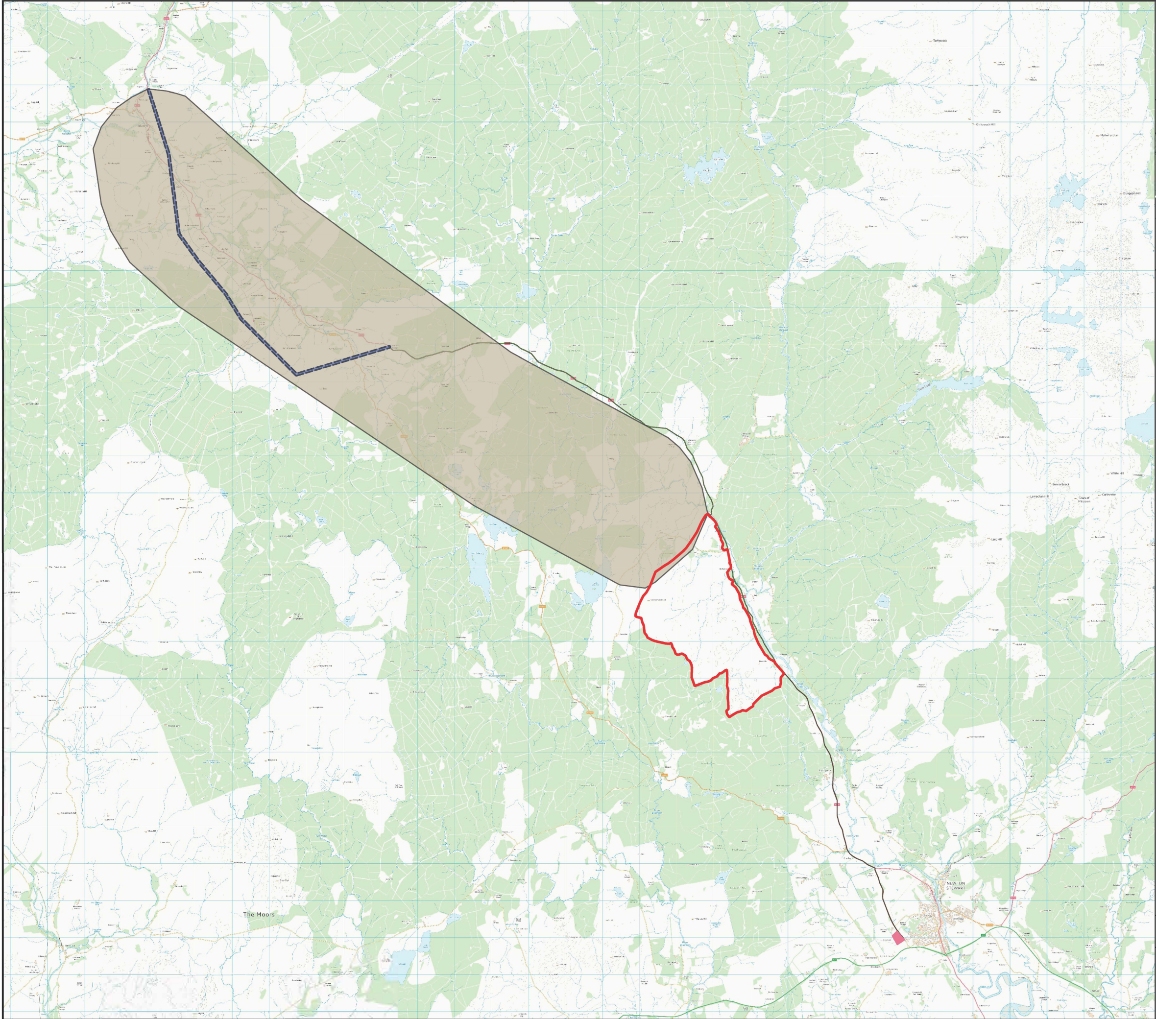
Figure 4.1: Indicative Grid Connection Routes and Overhead Line Area of Search
