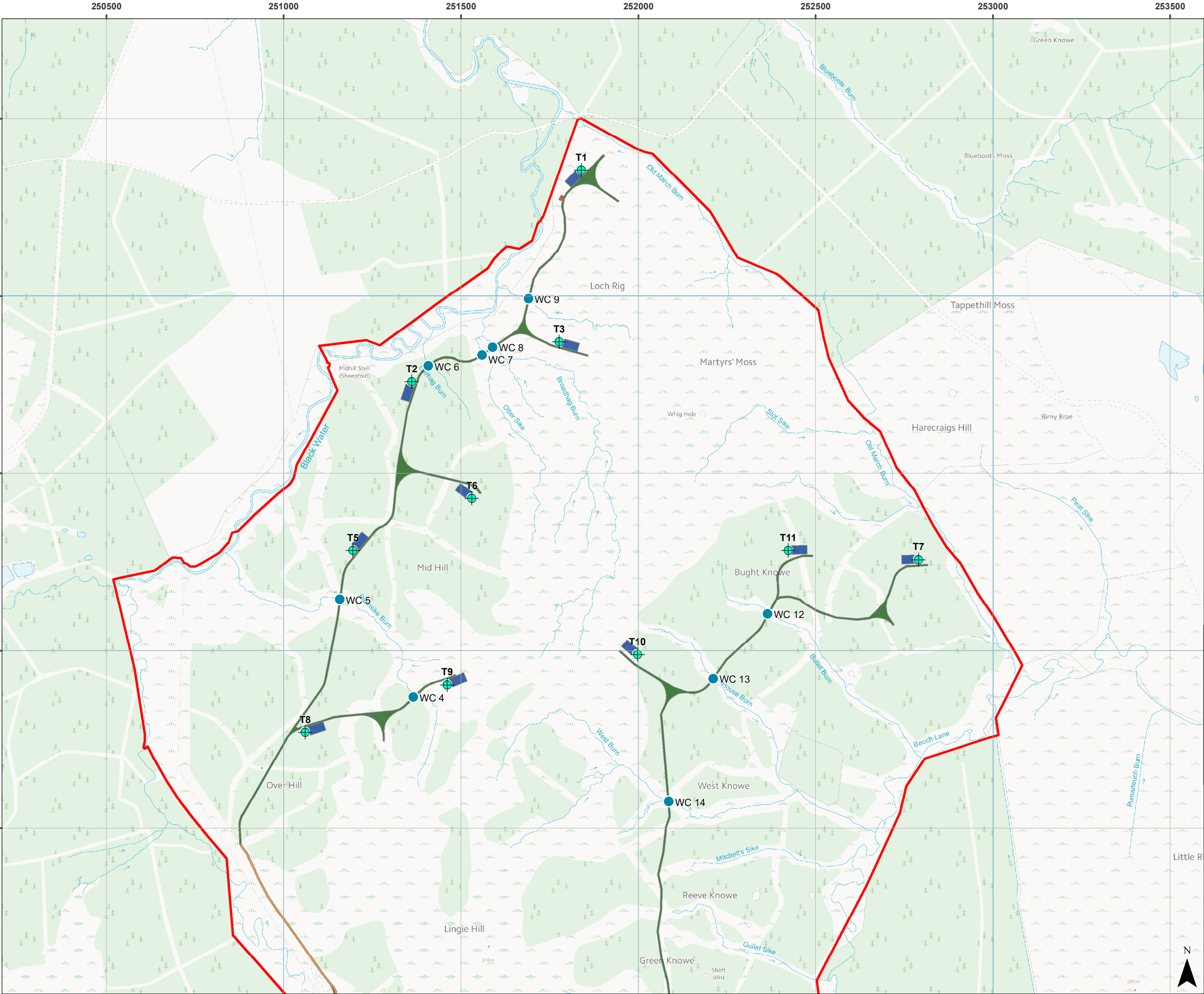
Figure 4.1a Proposed Development Layout
