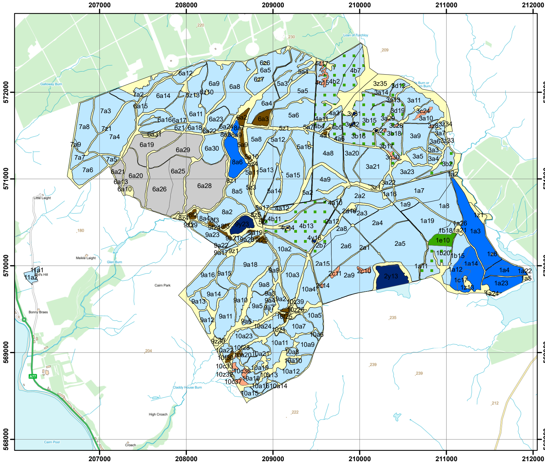
Figure 13.1: Loch Ree Forest - Compartment Plan in 2023
