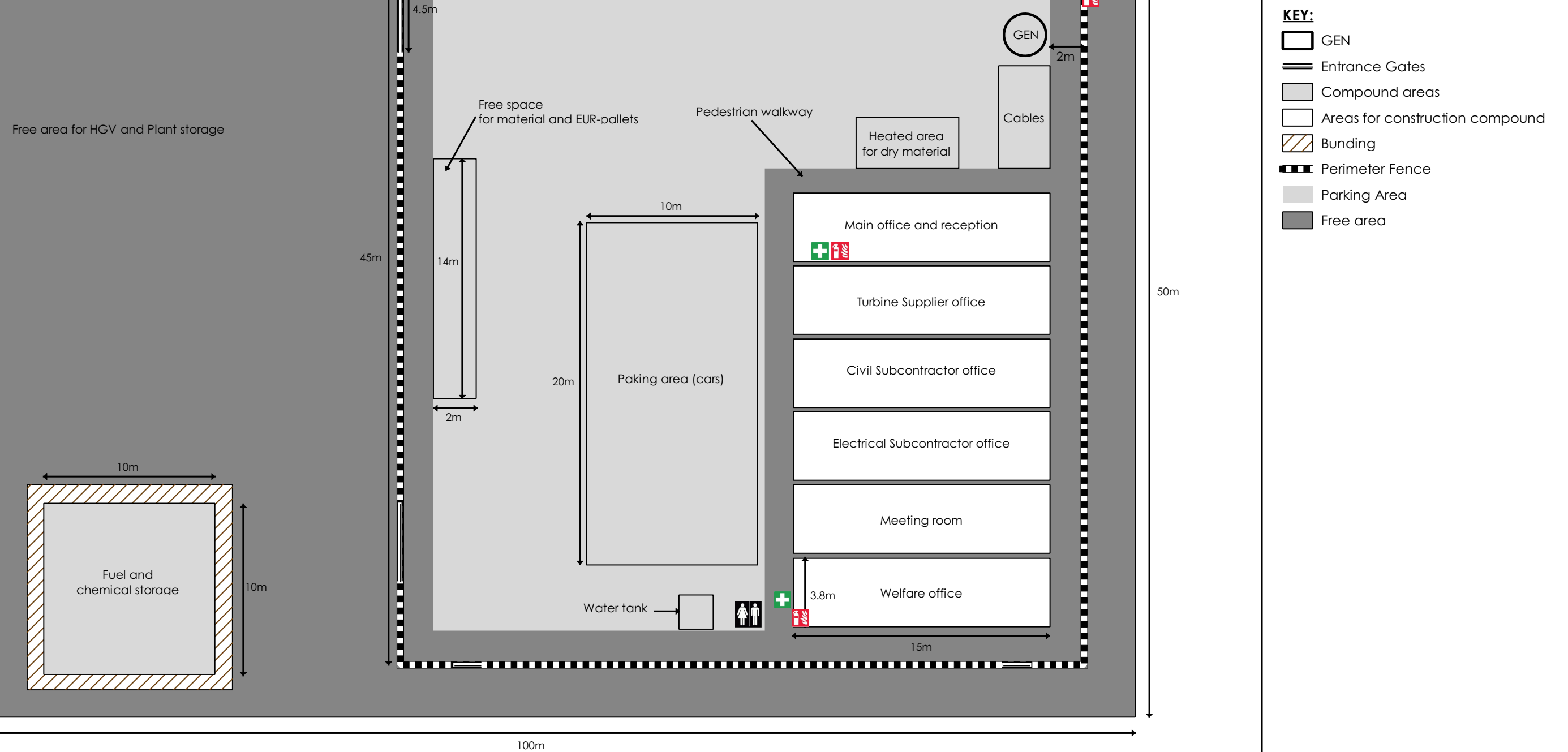
Figure 3.6: Typical Construction Compound
