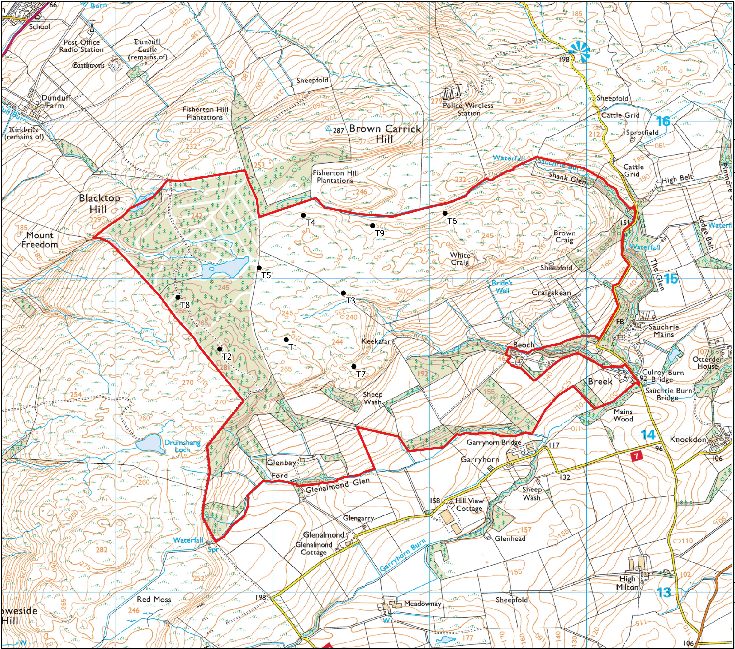
Figure 1.2: Indicative Turbine Positions
