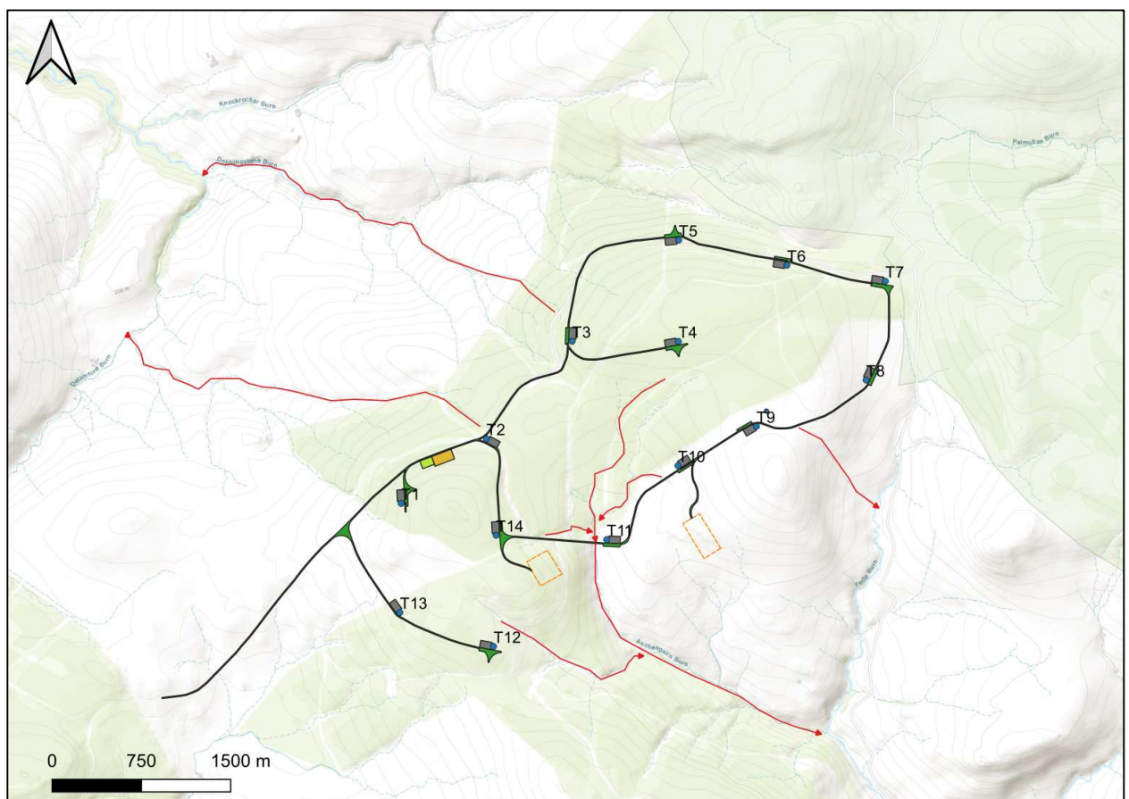
Figure 4.1: Peat Slide/Debris Flow Run-Out Pathways
